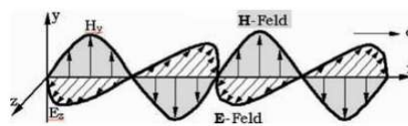
Figure 6. The planar electromagnetic wave in the far zone.
